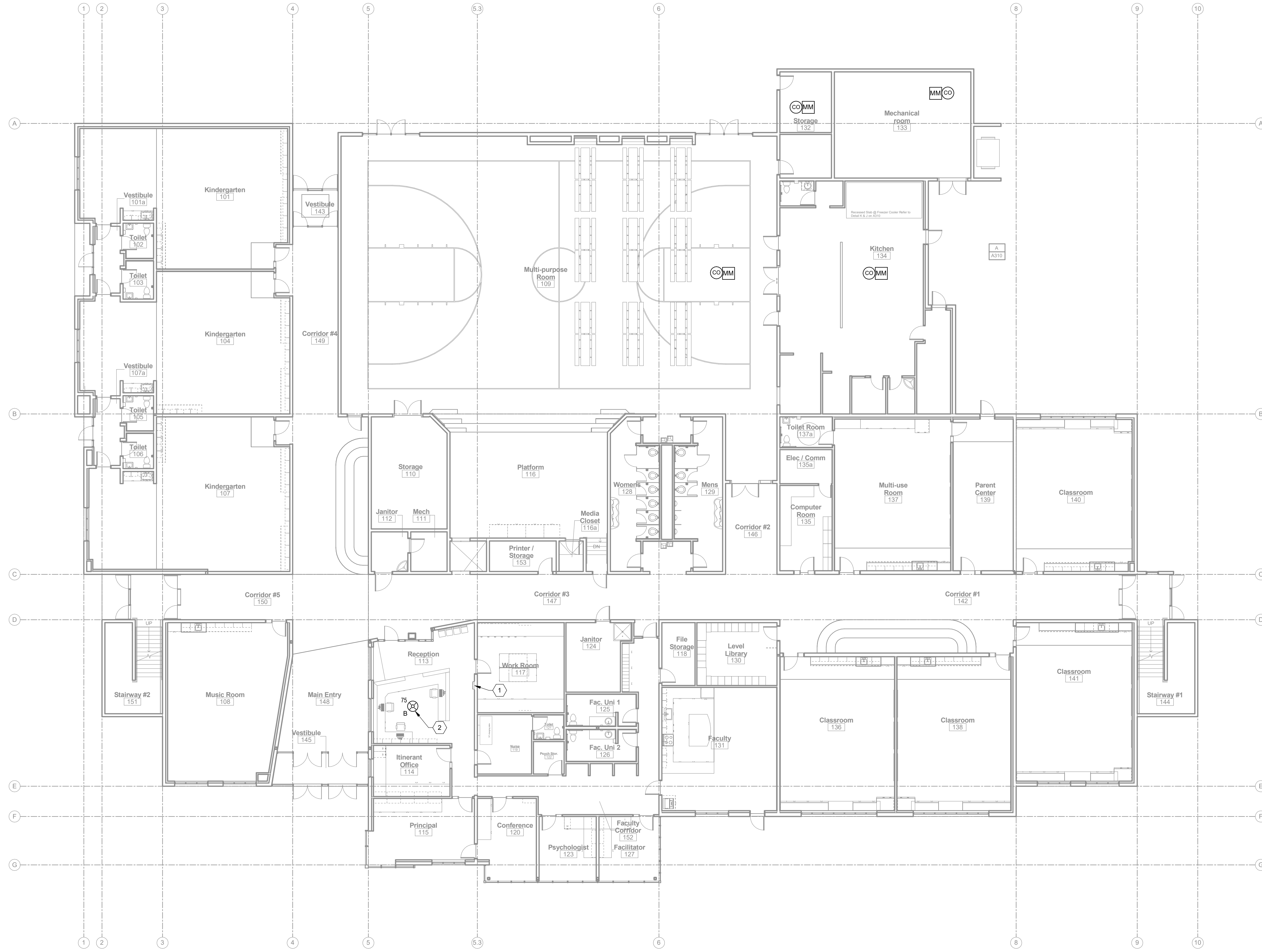
A1 CARBON MONOXIDE MONITORING PLAN - TIMPANOGOS SCALE: 3/32" = 1'-0"
